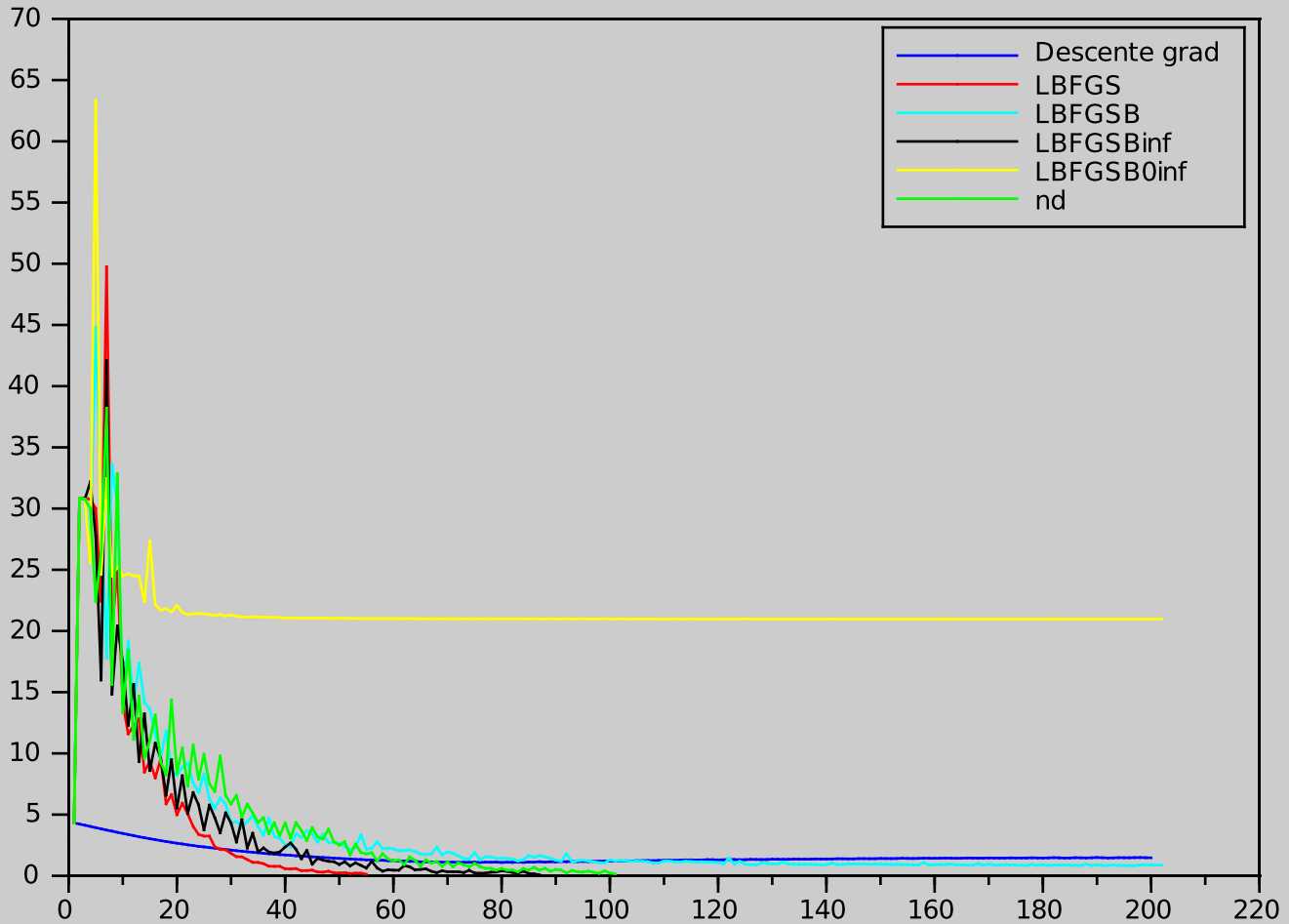
Gradient norm vs # function calls
