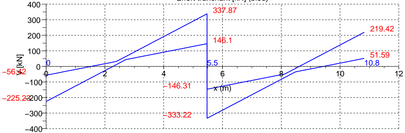
COURBE ENVELOPPE Effort tranchant [kN] (bleu)
