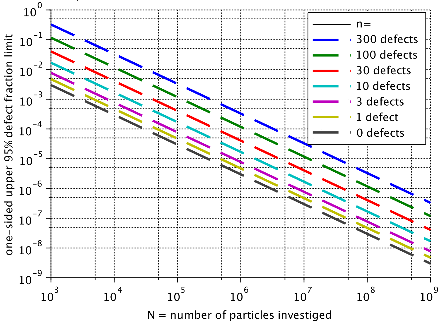
Acceptance limit of defect fraction n/N at 95% confidence
